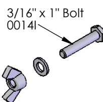
1.0" Rail Fixing Bolt Assem.
