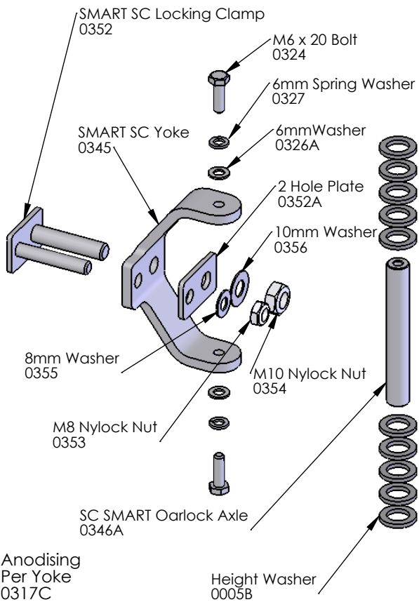
Sculling SMART Yoke Complete 0345A
